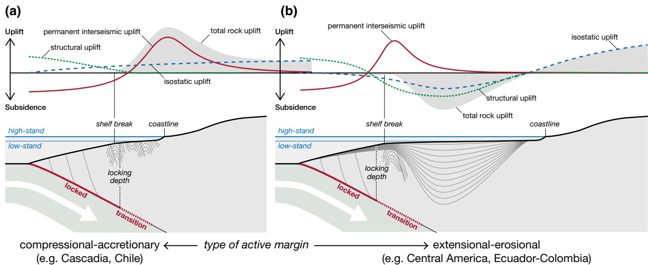
Figure 4. Conceptual model linking the morphology of active margins with the pattern of seismic coupling on the megathrust. (a) Contractional-accretionary forearc end-member ( sensu Noda, 2016). The combined patterns of permanent interseismic, isostatic, and structural uplift set the edge of the erosive shelf, landward of which rock uplift exposes bedrock to wave-base erosion (top). The shelf break lies close to the location of the downdip edge of high coupling, pinned by the locally strong gradient in interseismic uplift. The shelf grows landward from the edge by coastal retreat (bottom). (b) Extensional-erosional end-member (erosion refers to subduction erosion here). Here, subsidence of the wedge overcomes permanent interseismic uplift (top) and uplift at the shelf break acts as a sill for the forearc basin (bottom).
